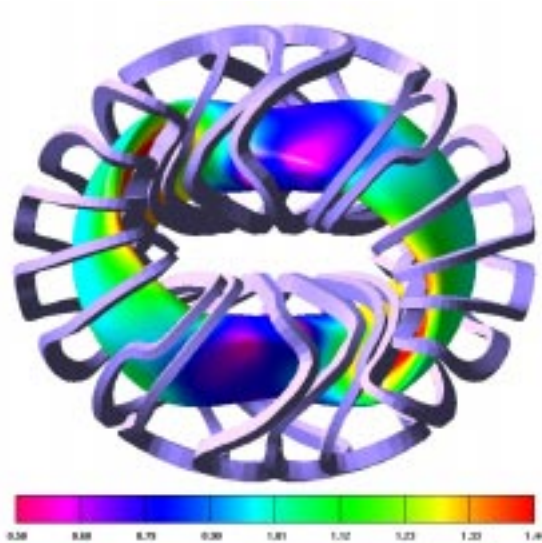
Fig. 1. Top (left) and side (above) views of the QPS plasma and the modular coils used to create it. The colors indicate contours of constant |B|(T) on the last closed surface.
