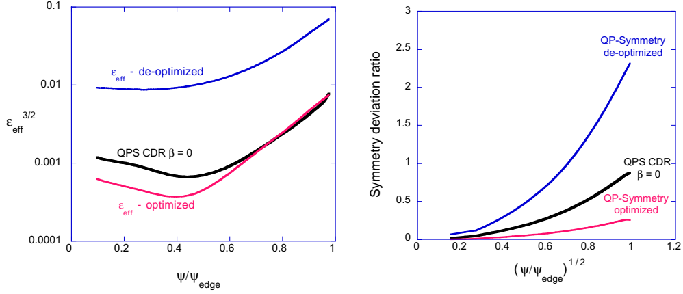
Fig. 3. Changes in the QPS coil currents permit varying (a) neoclassical transport and (b) quasi-poloidal symmetry over a wide range.
