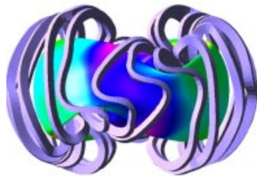
Fig. 1. Top (left) and side (above) views of the QPS plasma and the modular coils used to create it. The colors indicate contours of constant |B|(T) on the last closed surface.
