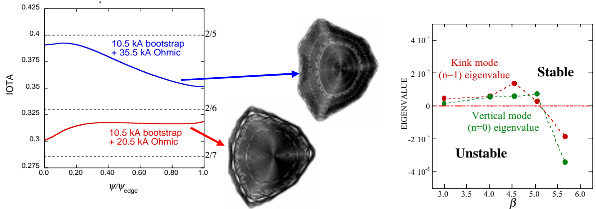
Figure 4. (a) Rotational transform profiles and flux surfaces in the D-shaped cross section at \langle\beta\rangle = 2\% ; (b) eigenvalues for n = 0 and n = 1 modes.
